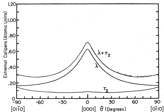
FIG. 17. Comparison of calculations and data for \lambda + \tau_2 signal.
